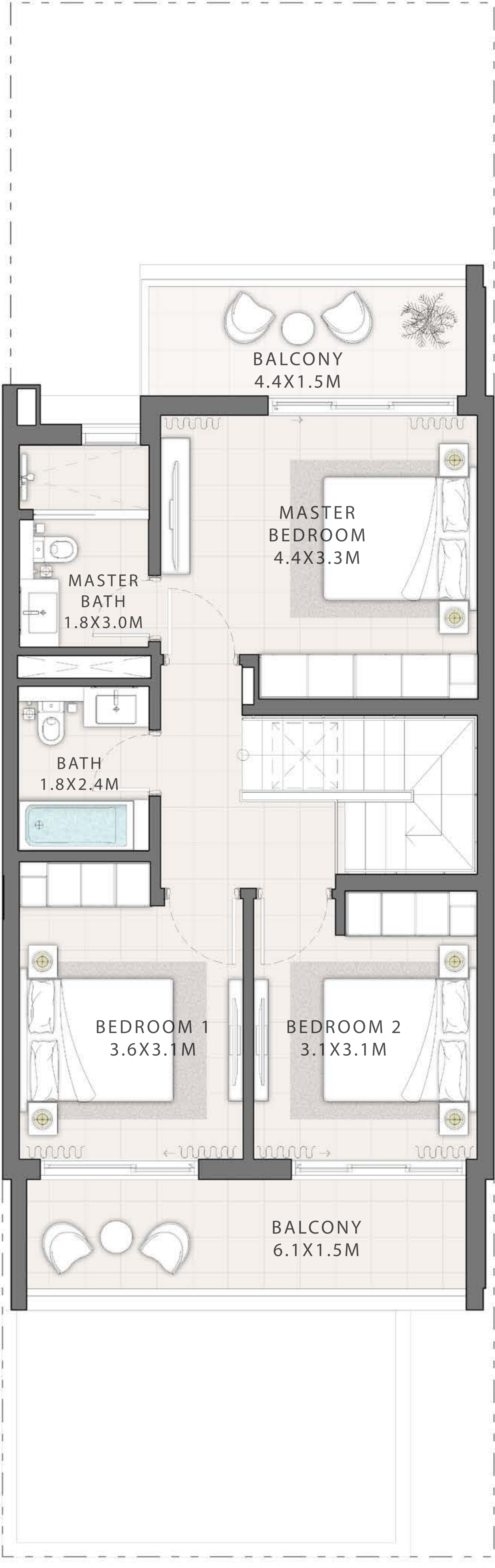
FIRST FLOOR
