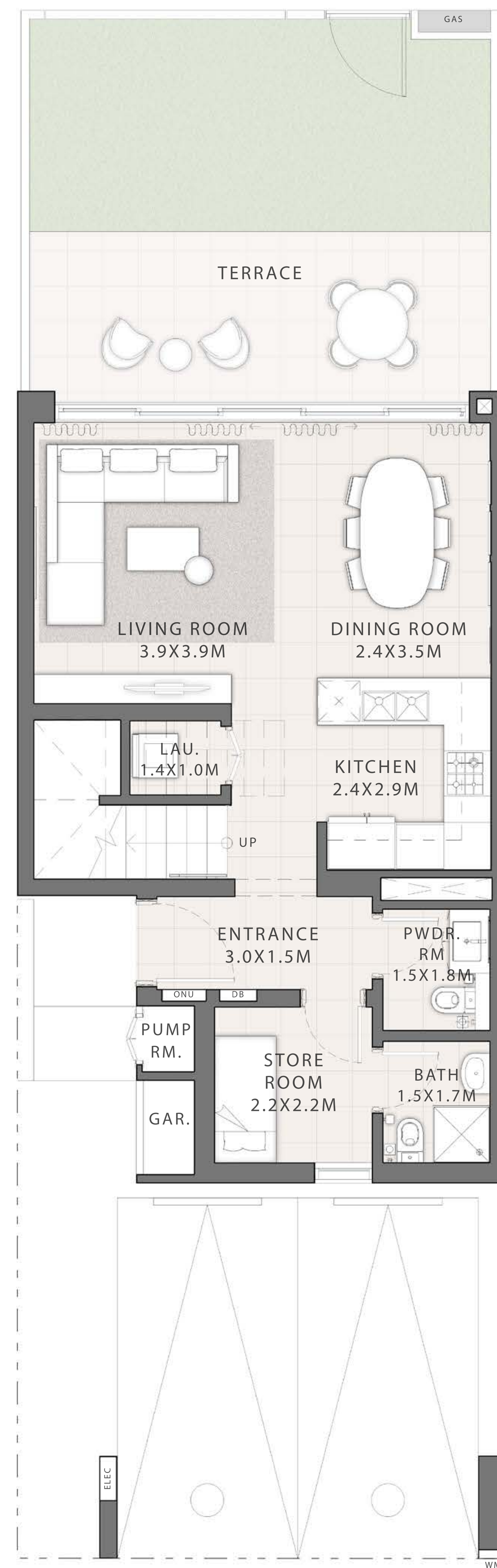
GROUND FLOOR
